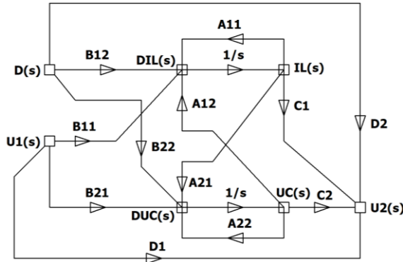
Fig. 15: Signal flow graph of a second order converter
