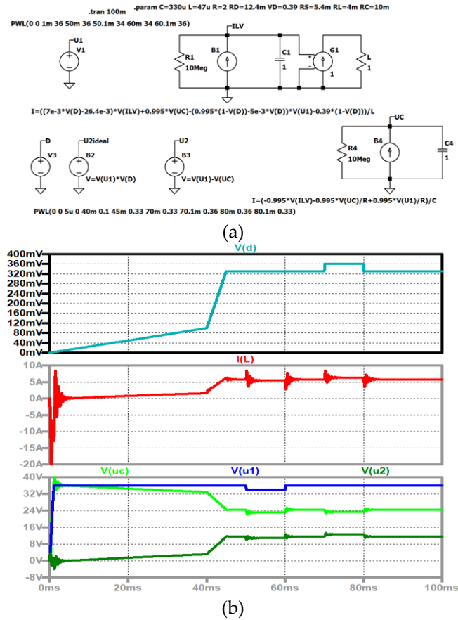
Fig. 22: Model with parasitic resistors: inrush, start-up, duty cycle steps, input voltage steps: (a) simulation circuit; (b) top to bottom: duty cycle (turquoise); current through the coil (red); input voltage (blue), voltage across the capacitor (green), output voltage (dark green)
