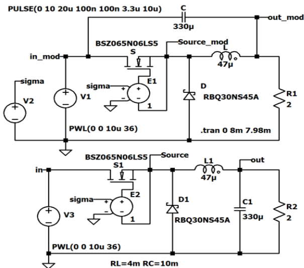
Fig. 26: Simulation circuit
