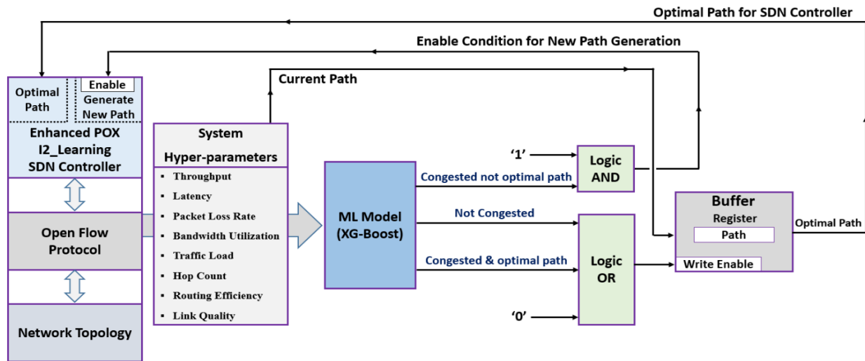
Fig. 2: Proposed Integration of ML with the enhanced I2_learning POX controller
