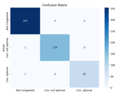
Fig. 3: Testing set generated XG-Boost model CM
