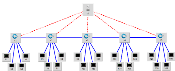
Fig.1: Main topology
